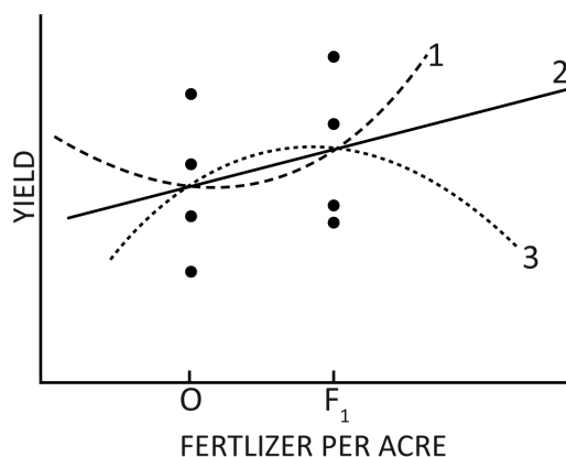
Figure 2 - Hypothetical data and estimated quadratic function
