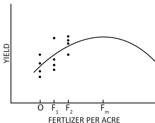
Figure 1 - Hypothetical data and three estimated quadratic functions
