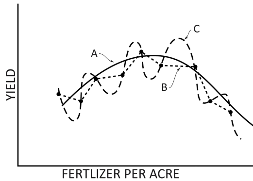
FIGURE 3 - HYPOTHETICAL DATA AND THREE ESTIMATED FUNCTIONS
